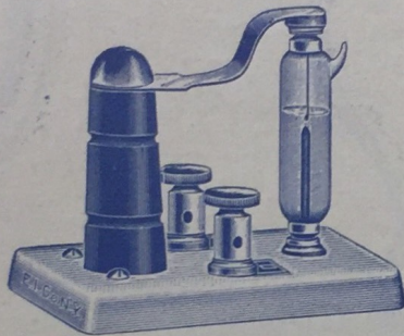
The "Radioson" Detector.
