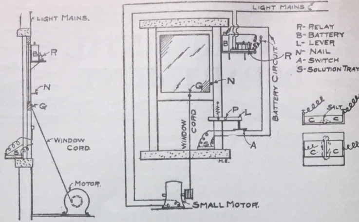
Automatic Window Closer
