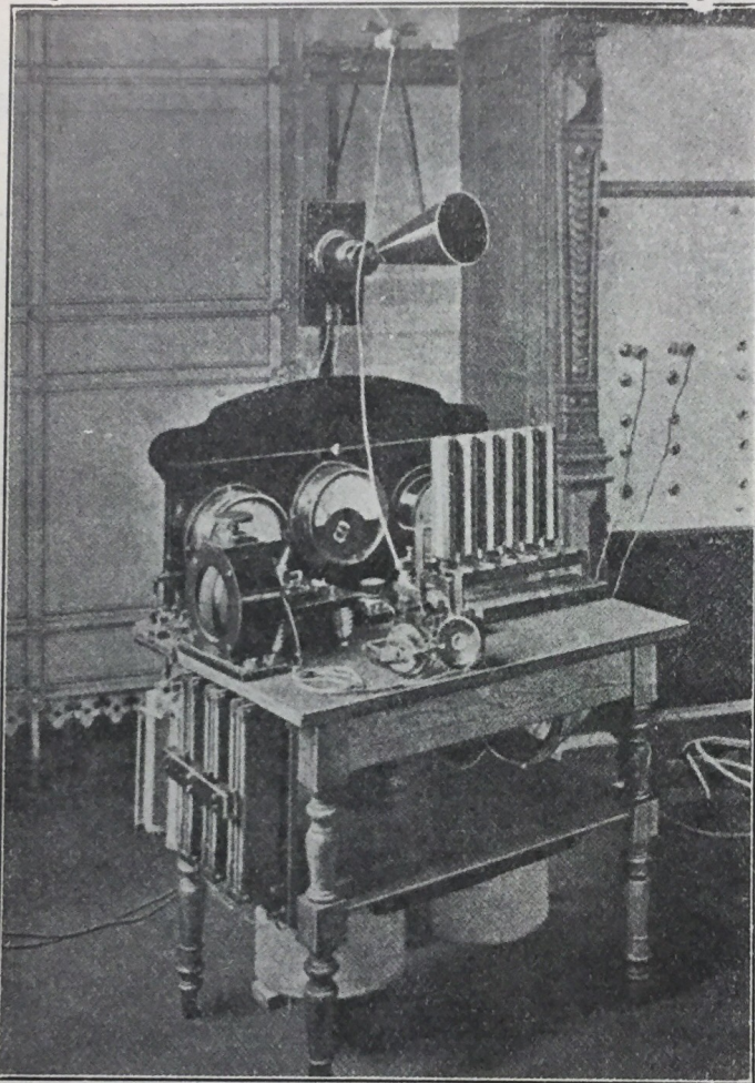
A WIRELESS TELEPHONE STATION
