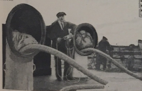
Photo shows hoses lowered into hold of ship through the ventilators. Hose delivers carbon monoxide which kills rats.
