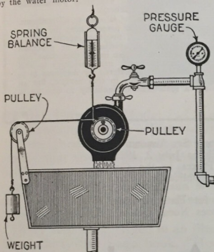
The set-up of the apparatus for determining the horse-power of a water motor.
