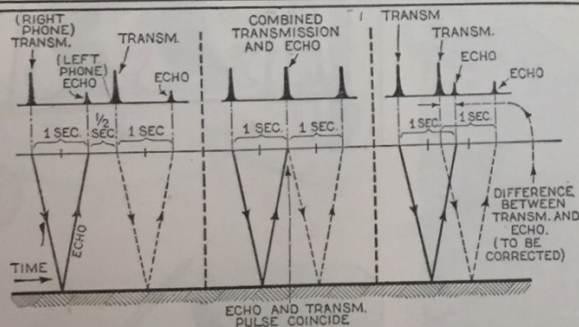
A schematic diagram of the sound wave depth finder. Sound waves strike ocean bottom and time taken for echo to be received is accurately measured.
