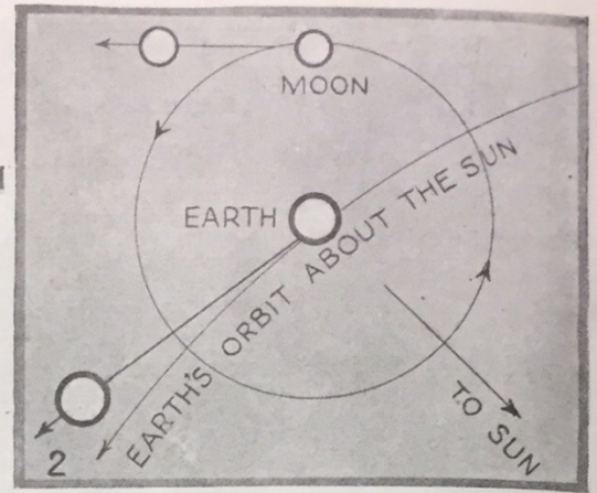
Fig. 2 above shows what would happen if the force of gravity suddenly refused to act. The earth and moon would fly off into space at a tangent to their orbits, as indicated by the straight arrows. The effect is the same as when a small boy is swinging a weight on the end of a string around his head and the string breaks. The weight, travels off in a straight line at a tangent to the path it traveled when confined by the string. Observations, however, show no weakening in the force of gravity.
