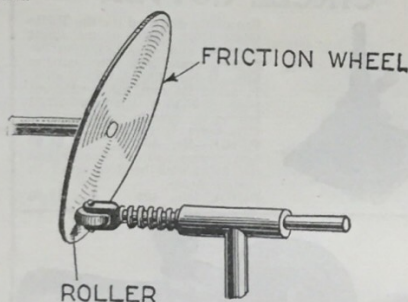
Simple form of variable cam.
