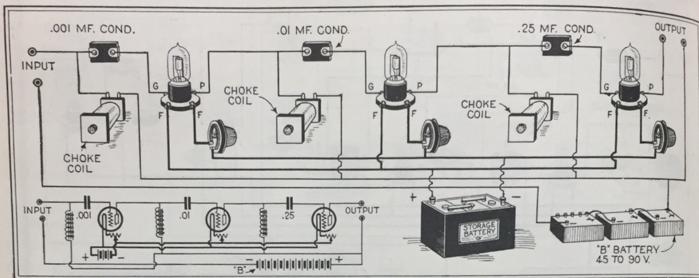
The choke coils in the above circuit may consist of approximately 10,000 turns of No. 36 enameled wire, wound on a 1/2-inch iron wire core 3 inches long. Suitable end plates should be provided. If desired, the secondaries of small spark coils may be used as the chokes.
