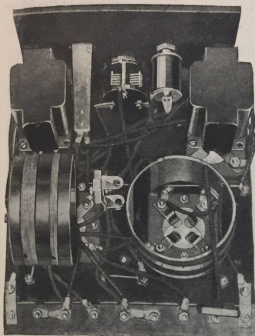
The above photo shows the bottom view of the assembled four-tube portable receiver. Note the compact arrangement of parts. The midget condenser in the center of the front panel serves to equalize the radio frequency and detector circuits. To the right of the condenser is the filament switch and to the left is the jack which is placed in the first stage of audio frequency amplification.
