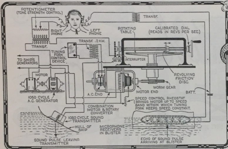
A schematic diagram of the sound wave depth finder. Sound waves strike ocean bottom and time taken for echo to be received is accurately measured.
