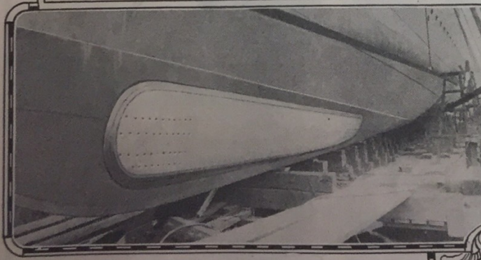
Steel "blister" on the S.S. Niagara placed below the water line, which houses the microphones.
