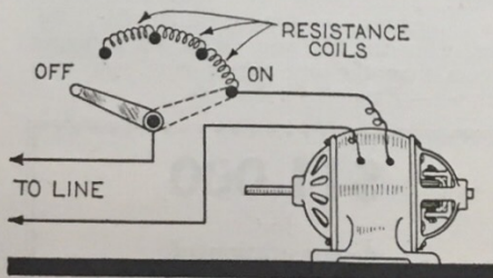
How the resistance coils in a small motor starting box are connected and used.
