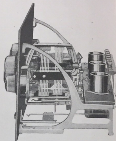
The efficient three-tube, three-circuit tuner detailed on this and the two succeeding pages is shown at the left and above. The numbers on the photographs at the left are carried through this entire article. The mounting brackets shown in the above photograph are a manufactured product.
