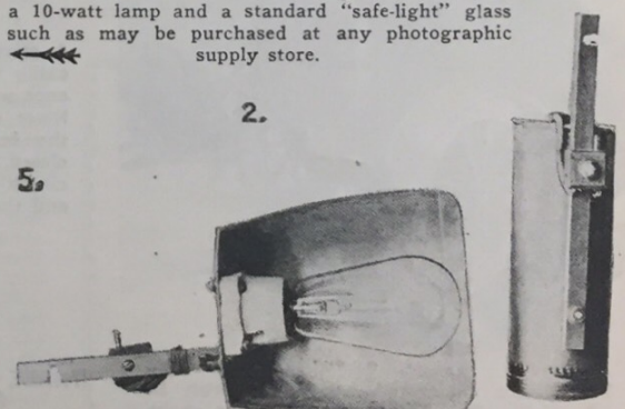
Above: Work lamp with half tin can as reflector.
